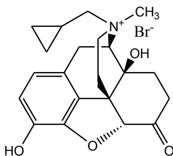
Figure 1: Methylnaltrexone bromide – Structure
